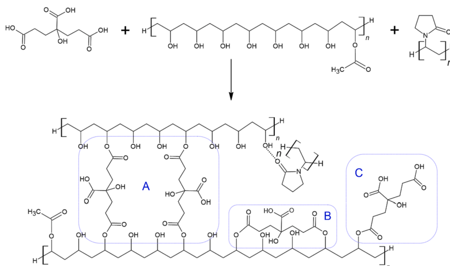
Fig. 2. Proposed crosslinking reaction mechanism speculating the position of citric acid after thermal treatment and how PVP interacts with the rest of the polymer.
